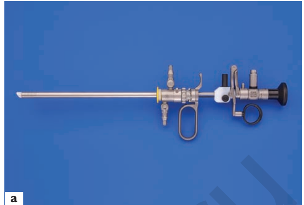
Figure 40.5 Bettocchi hysteroscope: close-up with 3.8 mm and 4.5 mm outer sheath system
