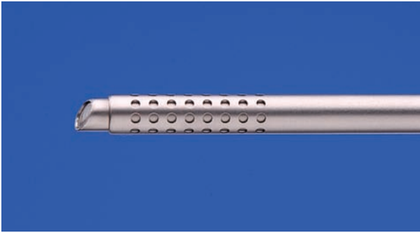
Figure 40.5 Bettocchi hysteroscope: close-up with 3.8 mm and 4.5 mm outer sheath system
