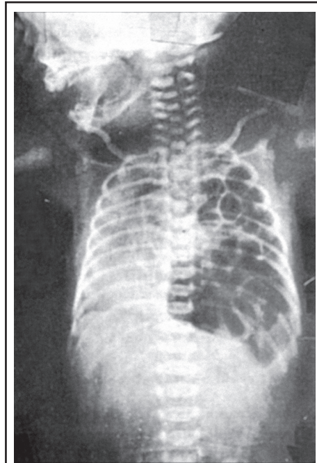
Fig. 32.9: Diaphragmatic hernia
